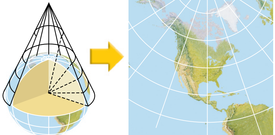
Figure 4 A light at the center of a transparent globe would project lines on a paper cone (left) that would produce a conic projection (right).
